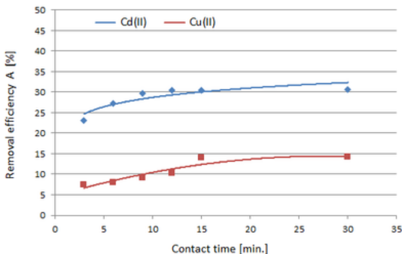
Figure 3. The effect of contact time on Cu(II) and Cd(II) adsorption (initial concentration 100 mg/L; initial pH 2; mass of adsorbent 100 mg).
