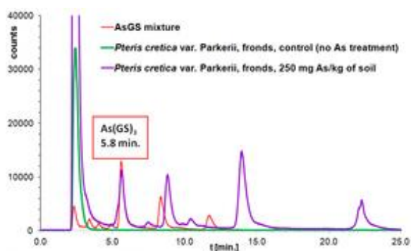
Fig. 1. Chromatographic separation of an extract of Pteris cretica var. Parkerii grown for 90 days in 250 mg arsenic per 1 kg soil.
