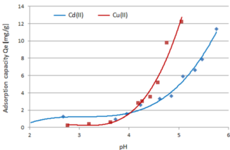
Figure 2. The effect of pH on Cu(II) and Cd(II) adsorption (initial concentration 100 mg/L; contact time 30 min.; mass of adsorbent 100 mg).
