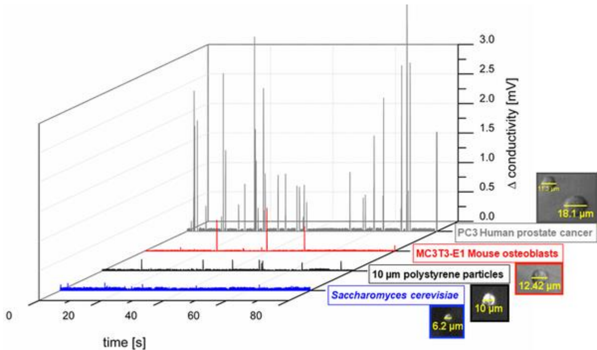
Fig. 2: Resistive pulse signals of PS particles and biological cells.
