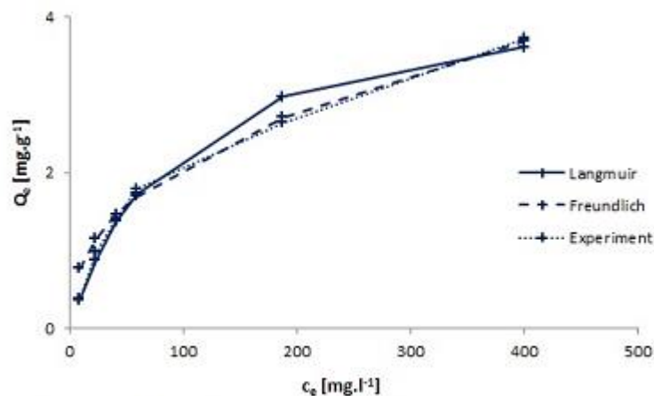
Fig. 5. Sorption isotherms of Cu(II) using grape waste. pH value: 4; contact time: 30 minutes
