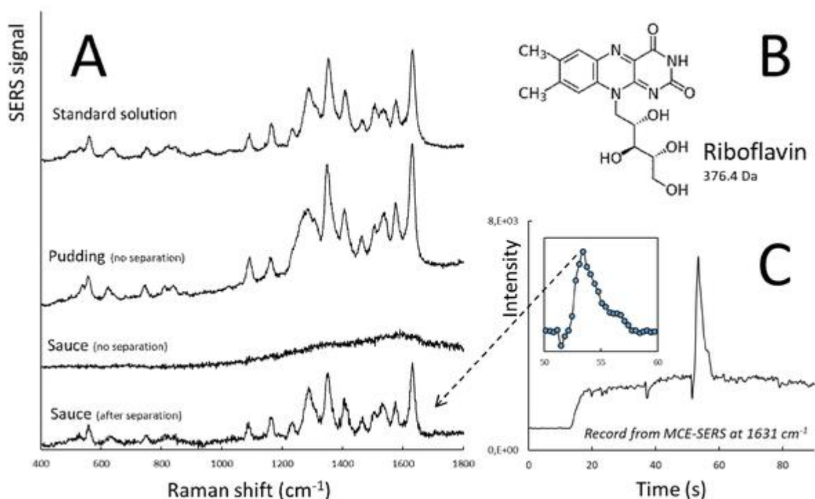
Fig. 3: A - Various samples containing riboflavin analysed from a droplet or online as a zone after MCE separation. B - Structure of riboflavin. C - MCE-SERS record of analysis of barbecue sauce. The inserted window shows frequency of data points.
