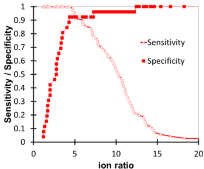
Figure 3. The dependence of sensitivity and specificity of the method on the ion ratio values.
