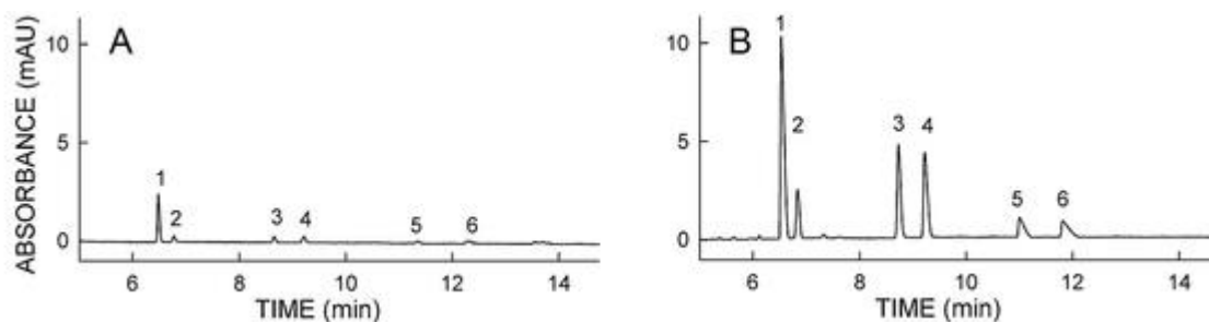
Fig. 3. Separation of methadone and EDDP enantiomers in presence of romifidine and D-(+)-norephedrine. Injection and separation voltage was 8 and 20 kV, respectively. Buffer plug length was 20 mm, BGE comprised 100 mM phosphate (pH 3) and 0.12% (w/v) of HS- \gamma -CD. (A) Buffer plug comprised 50 mM phosphate buffer (pH 3), injection time was 15 s. (B) 10-mm water plug was introduced prior injection, buffer plug comprised 100 mM phosphate buffer (pH 3), injection time was 30 s. Key: 1: D-(+)-norephedrine, 2: romifidine, 3: S-methadone, 4: R-methadone, 5: R-EDDP, 6: S-EDDP. Data are from [6].
