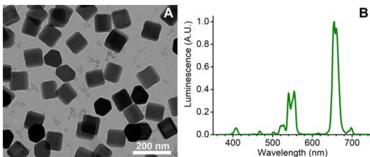
Figure 1. (A) Transmission electron microscopy of investigated UCNPs. (B) Emission spectra of nanoparticles recorded in 300 nL water droplet (nanoparticle concentration 7.5 pmol/L, integration time 100 ms).
