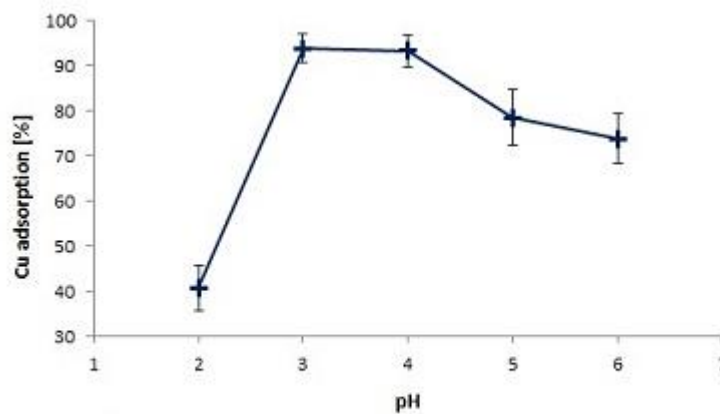
Fig. 3. Effect of pH on the copper adsorption onto grape waste. Initial metal concentration: 100 mg/l; contact time: 30 minutes
