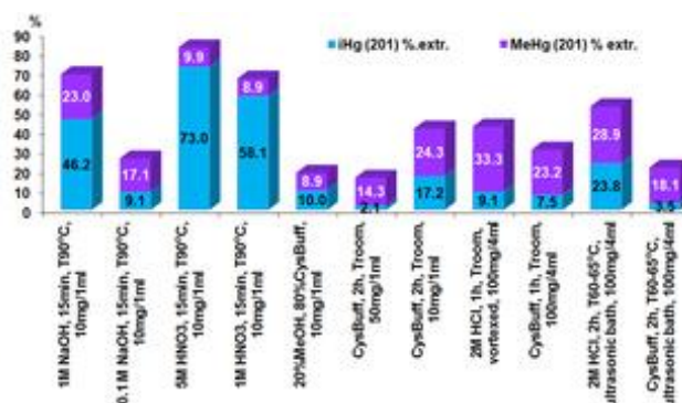
Fig. 2. The extraction yields of i\text{Hg}^{2+} and \text{MeHg}^+ obtained under various condition.
