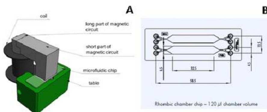
Fig. 1 (A) Scheme of home-made electromagnet from behanit with microfluidic chip (B) Scheme of Rhombic chamber chip with 120 \mu L.
