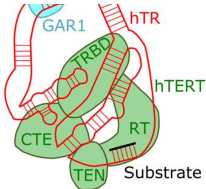
Scheme 2: Schematic of telomerase subunit catalytic core arrangements. hTR - RNA subunit of telomerase interconnects whole hTERT. Adapted from [8].
