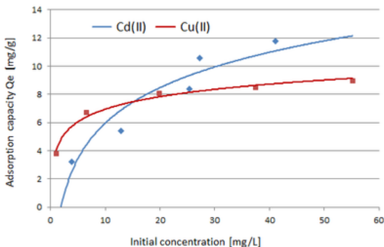
Figure 1. The effect of initial concentration on Cu(II) and Cd(II) adsorption (initial pH 2; contact time 30 min.; mass of adsorbent 100 mg).
