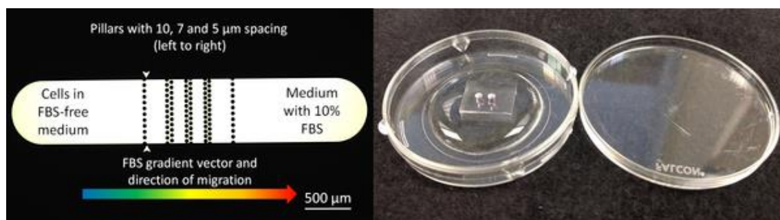
Fig. 1. Left - chromium mask for the fabrication of PDMS device. Right – assembled device used for confocal microscopy time lapse imaging.
