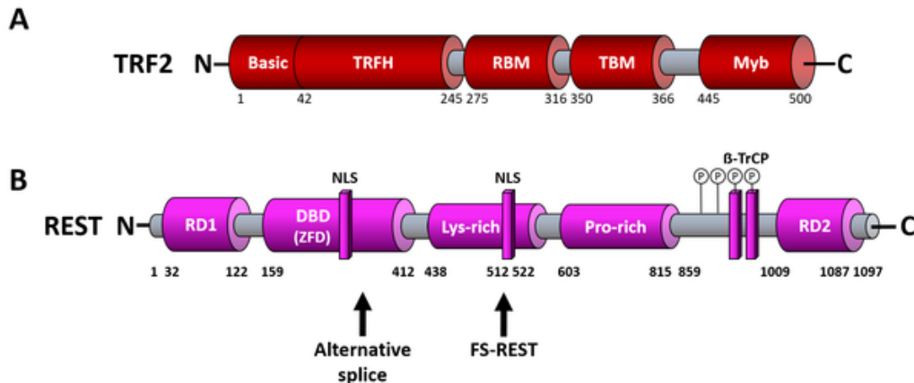
Figure 2: TRF2 and REST domain structure. A) TRF2 contains N-terminal basic domain (GAR), C-terminal DNA-binding Myb domain, TRFH dimerization domain; RBM–Rap1 binding motif, TIN2-binding motif TBM. B) REST consist of two repressor domains (RD1, RD2), DNA binding domain, lysine and proline rich regions and two \beta -TrCP binding sites. Arrows indicate truncated forms of REST that are associated with small-cell lung cancer and neuroblastoma (alternative splicing) or colon cancer resulting from a frameshift (FS-REST).
