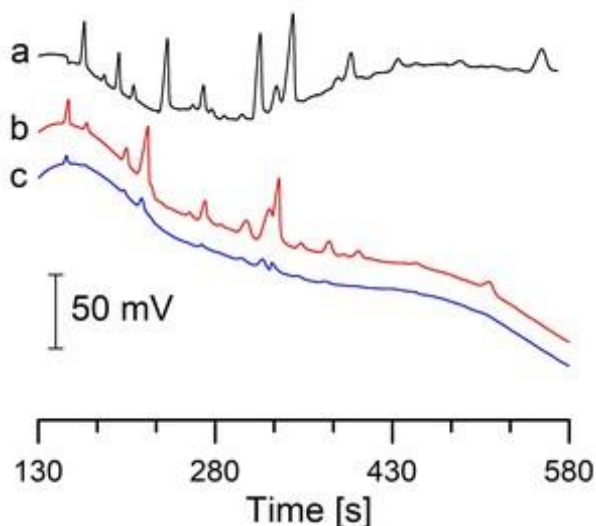
Fig. 1. Electropherograms from the analyses of brewed coffee sample in different BGEs. CE separations were carried out in the BGEs: 10 mmol/L MES, 1.2 mmol/L BisTris, 2.2 mmol/L BisTrisPropane, 0.1% HEC, 20 mmol/L \alpha -CD, 10 mmol/L \beta -CD, pH=6 (a), 35 mmol/L MES, 3.4 mmol/L BisTris, 6 mmol/L BisTrisPropane, 0.1% HEC, 20 mmol/L \alpha -CD, 10 mmol/L \beta -CD, pH=6 (b, c). The coffee sample prepared in espresso coffee machine was diluted 500 times (a, c) and 100 times (b). The constant separation current was stabilized at 30 \mu\text{A} (a) and 90 \mu\text{A} (b, c).
