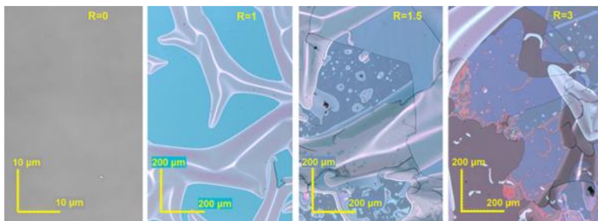
Fig. 1. Surface structure of chosen TMSA coatings after immersion in water.
