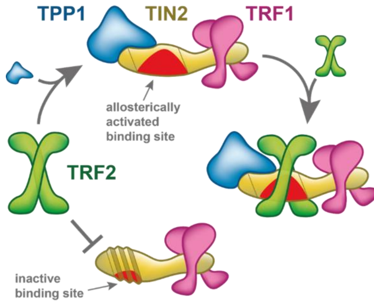
Figure 3: Model for sequential assembly of shelterin core complex. TRF1 prevents TRF2 from binding to TIN2 if TPP1 is absent, as TRF1 occupies the preferential binding site on TIN2 (lower part of the scheme). On the contrary, when TPP1 binds TIN2, TPP1 induced allosteric structural changes that open the second binding site on TIN2 and the binding site for TRF2 becomes active (upper part of the scheme). TRF2 binds TIN2-TPP1 along with TRF1 (middle part of the scheme). A stable shelterin core complex TRF1-TIN2-TPP1-TRF2 is formed.
